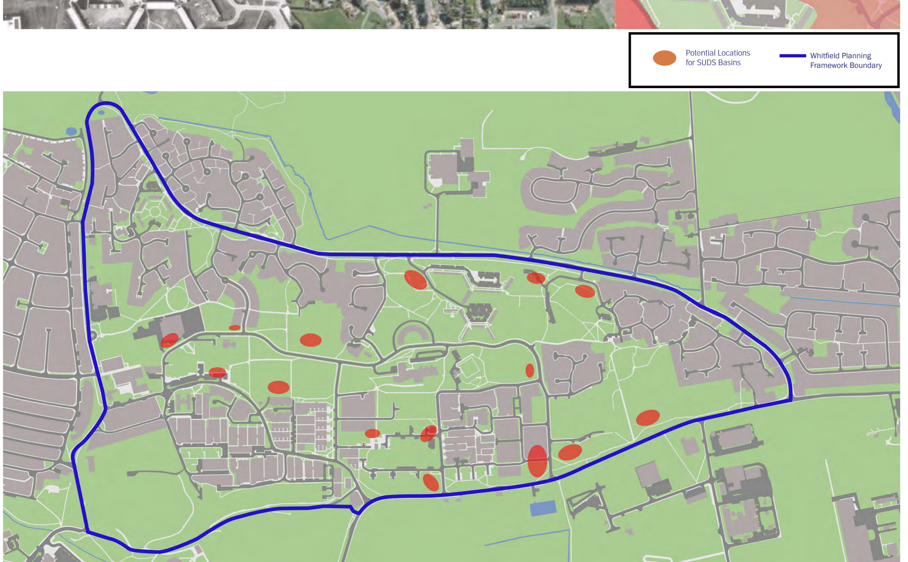
Figure 23: Map showing the potential location of SUDS basins (based on topography and other considerations) as part of the greater drainage infrastructure of Whitfield.
